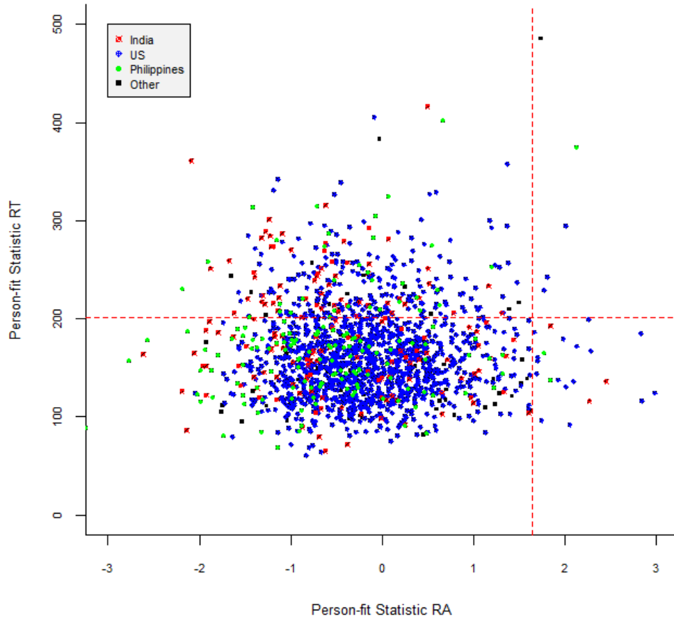
Figure 3: For different countries the person-fit statistic of RA patterns plotted against those of RT patterns.
