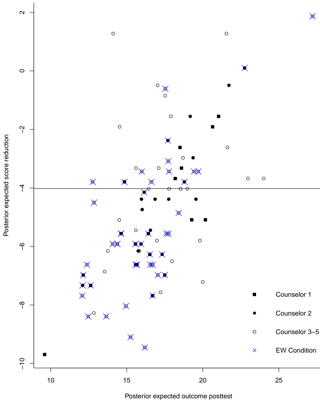
Figure 3. The email-counselling study from Lamers et al. (2015). Posterior expected post-intervention scores against the expected reduction in scores of clients across counsellors.
