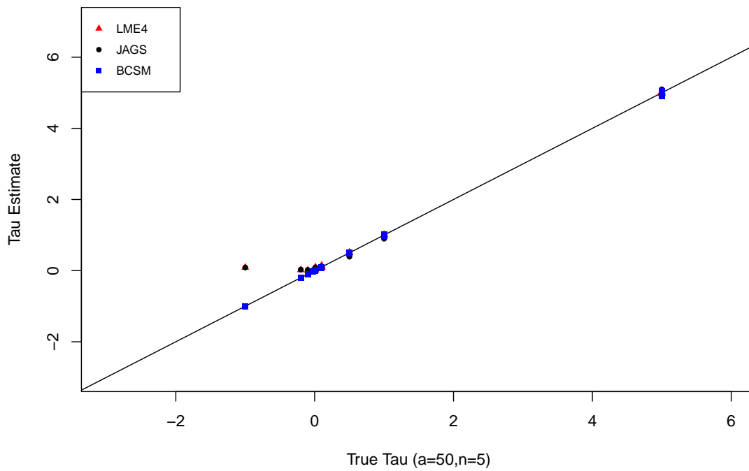
Figure 2. Averaged parameter estimates for \tau across 1,000 data replications under LME4, JAGS, and the BCSM.
