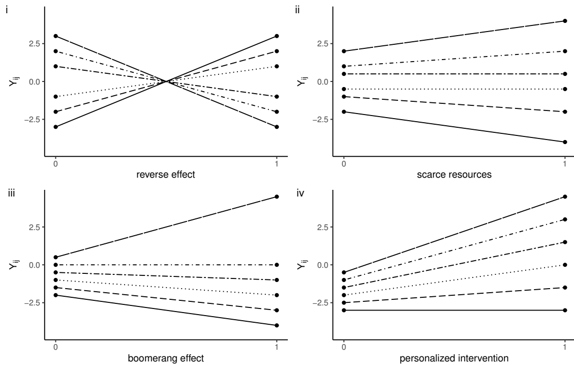
Figure 1. Four examples where the cluster variance \tau is negative (scenario i - iv). Outcome Y_{ij} , observed two times (e.g., repeated measures, 0 for the pre-, and 1 for the post-observation). Scenario i shows a reverse effect, all pre-observations are reversed ('reverse effect') at the post-measurement; ii shows a setting where individuals are competing for scarce resources (e.g., one's pain is the other's gain); iii shows how other group members decrease as a reaction to the increase of another group member ('boomerang effect'; Kenny et al., 2002); and iv shows that clustered individuals have dissimilar trajectories related to the personalized intervention.
