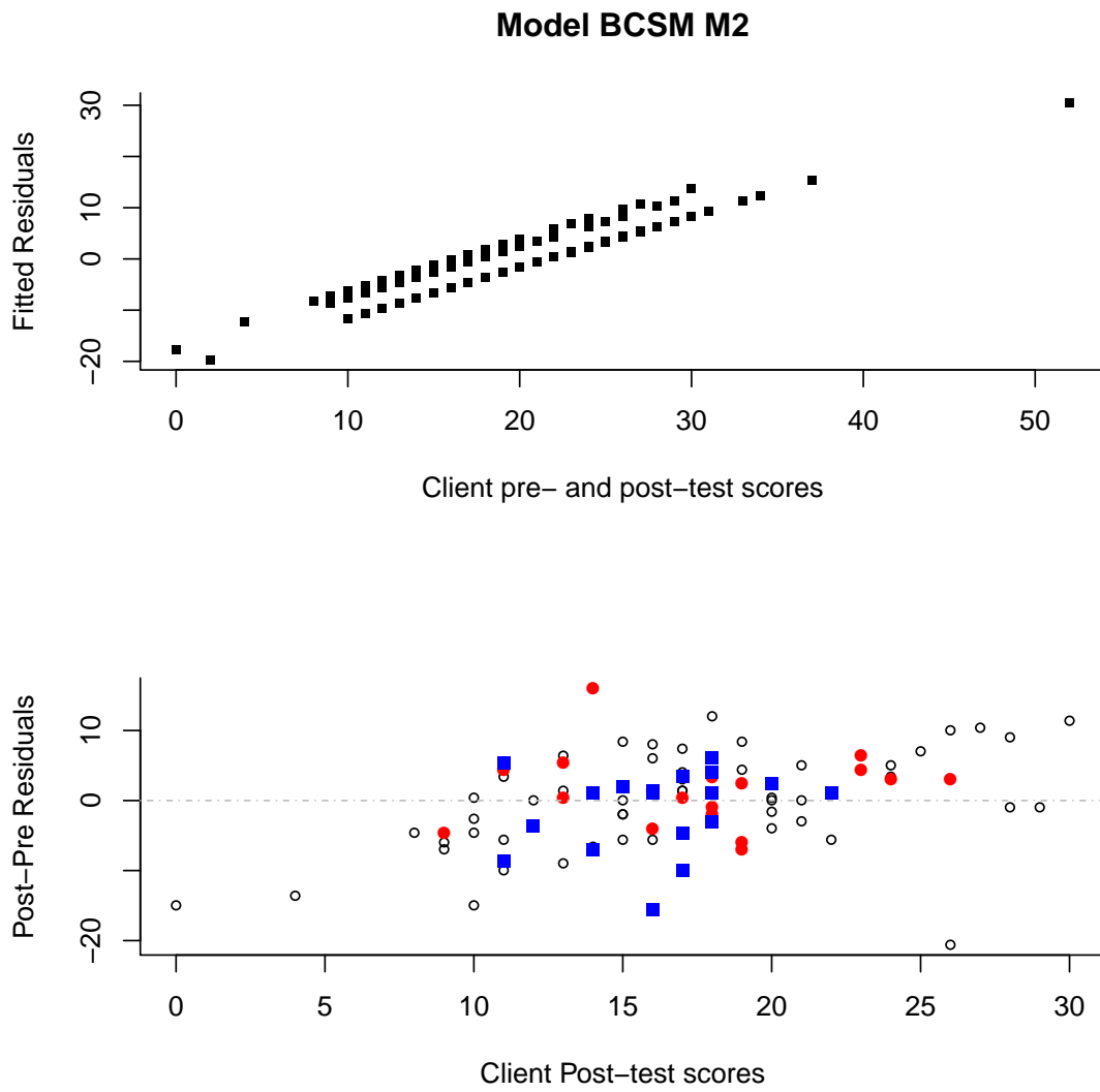
Figure 4. The fitted residuals under the BCSM M2, and the post-intervention scores against client’s post- minus pre-intervention residuals for different counsellors.
